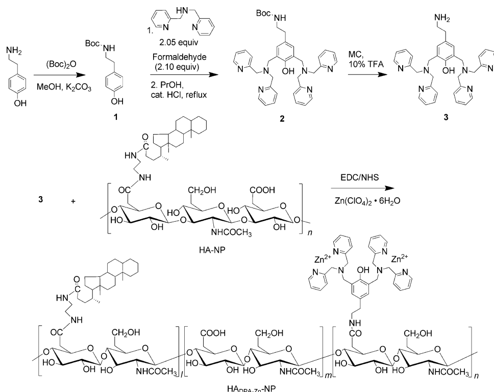
Scheme 1. Synthesis and chemical structure of HA DPA-Zn -NPs. Boc = tert -butoxycarbonyl, MC = CH 2 Cl 2 , TFA = trifluoroacetic acid.
